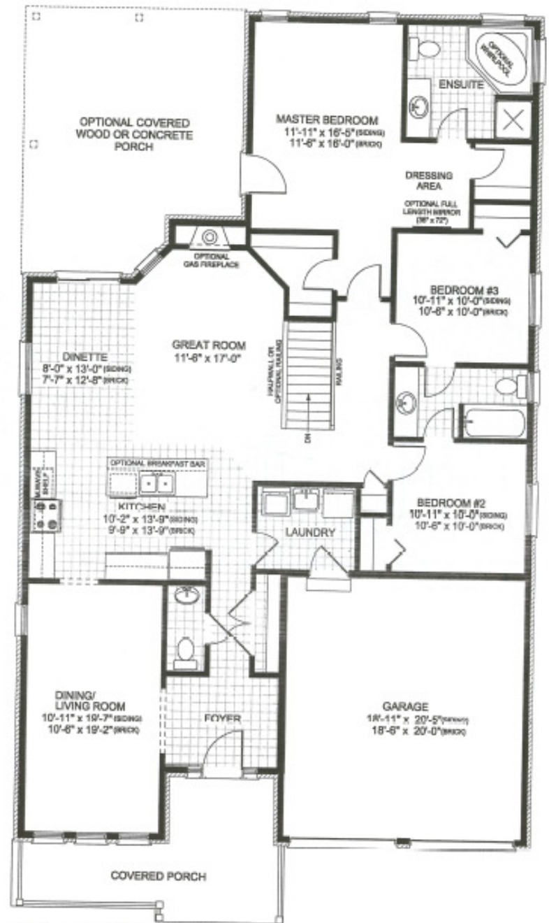
MAIN FLOOR PLAN 1804 SQ.FT.
