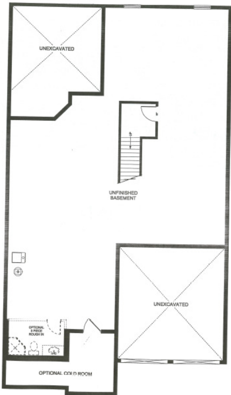
FOUNDATION PLAN
